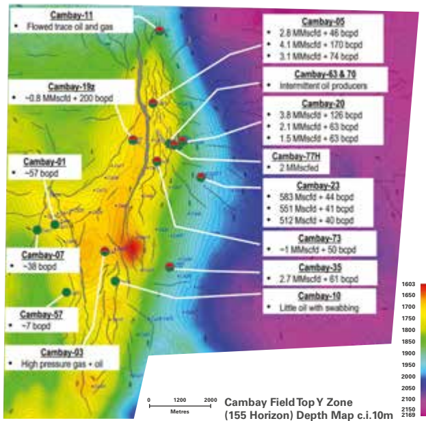
Figure 2 Cambay Field – recorded hydrocarbon flowrates from EP-IV (Y Zone) reservoir
